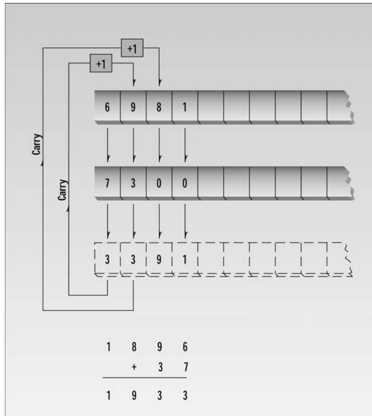
FIGURE 13.3 Adding verylong numbers.
